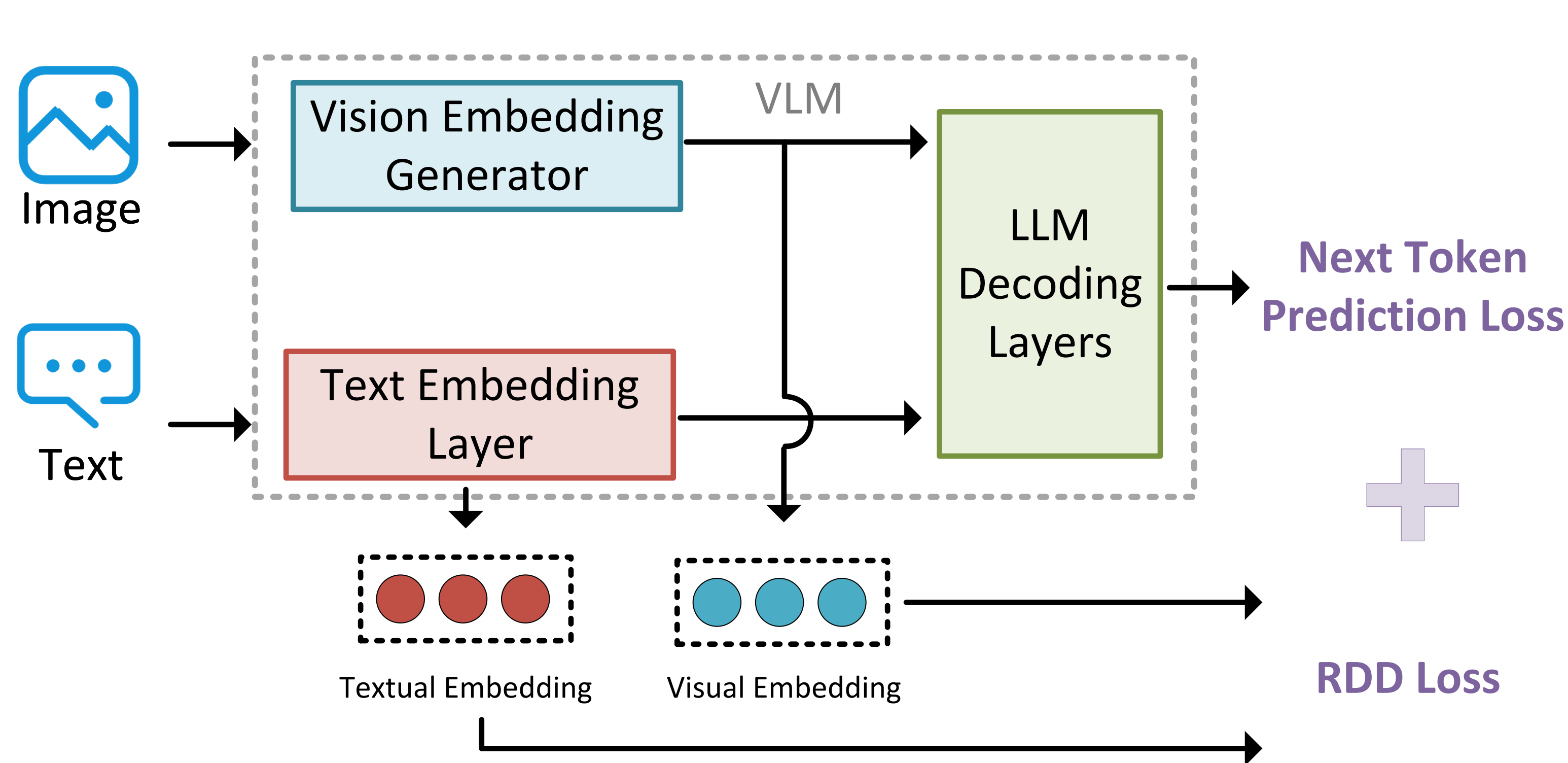
(a) Training Pipeline.
