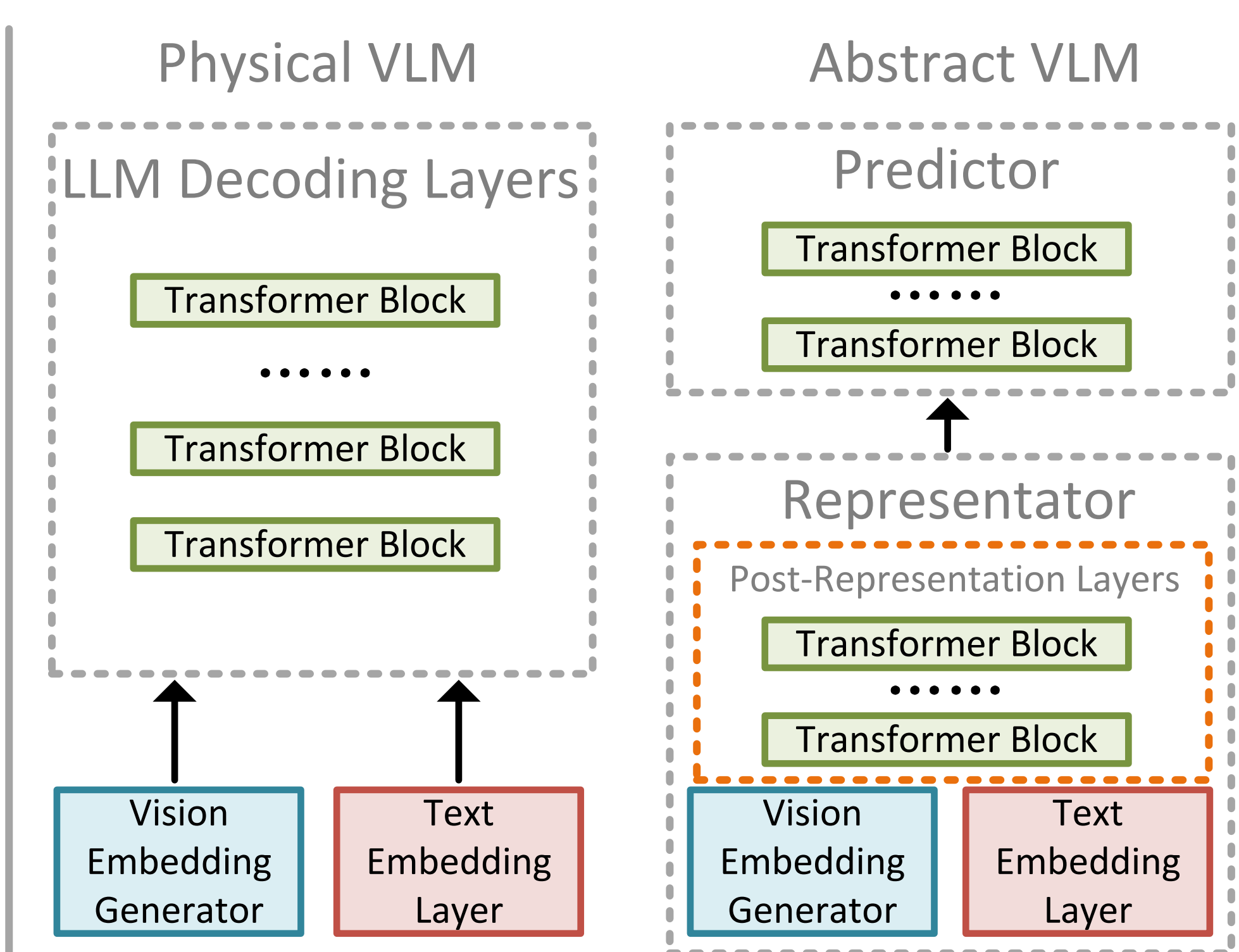
(b) Relation between the physical and abstract VLM.
